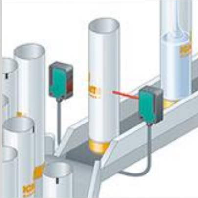
Thru-Beam Sensors
