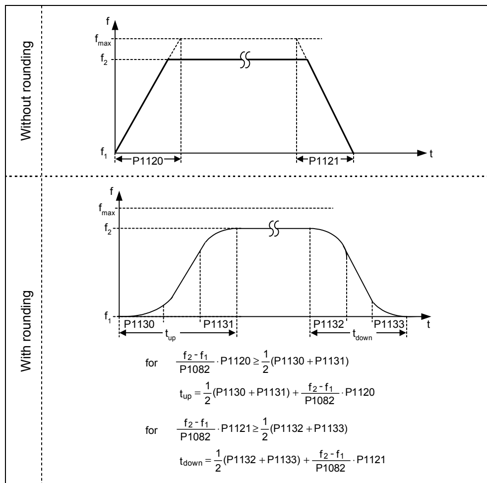
Fig. 3-62 Ramp-function generator
