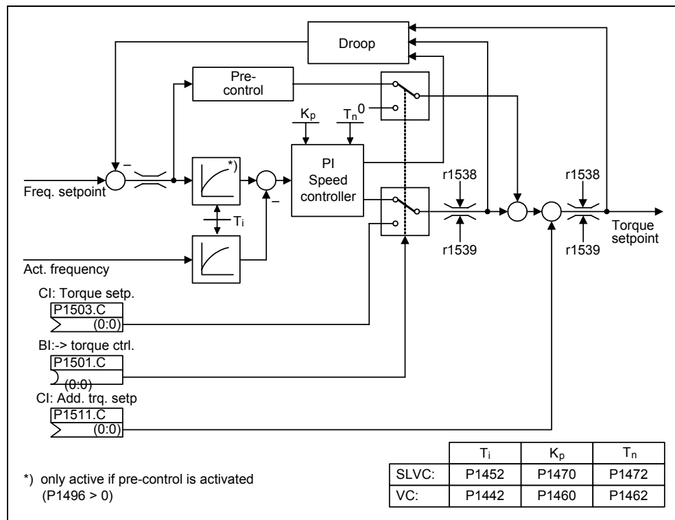
Fig. 3-108 Closed-loop speed/torque control
