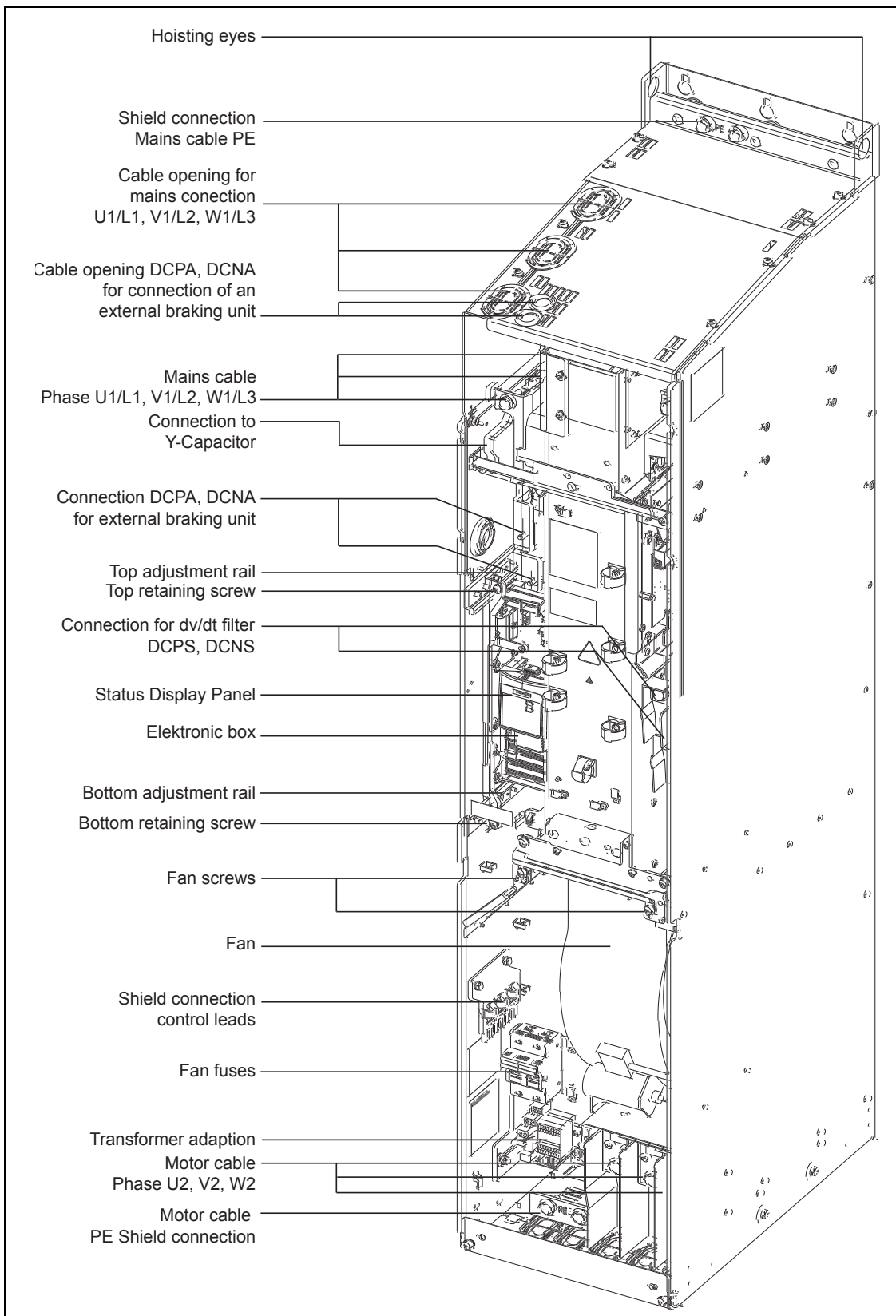
Fig. 2-10 MICROMASTER 440 connection drawing - frame size GX
