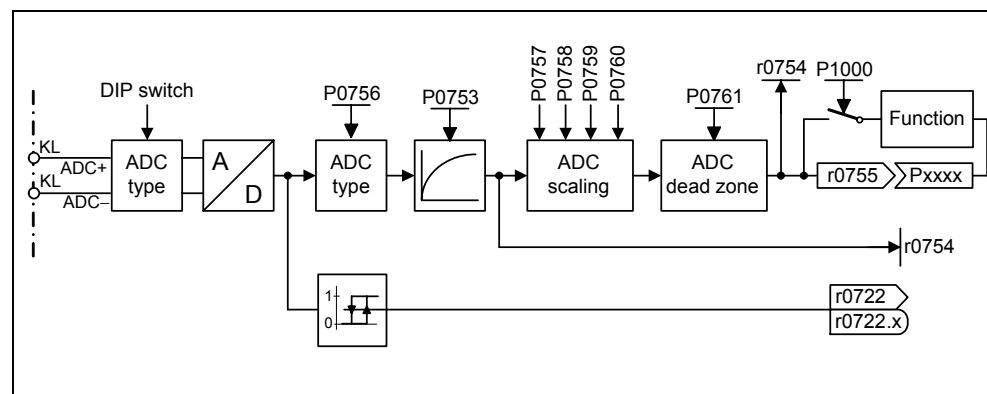
Fig. 3-33 ADC channel
