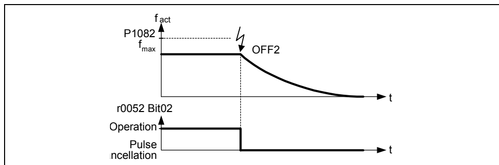
Fig. 3-65 OFF2
