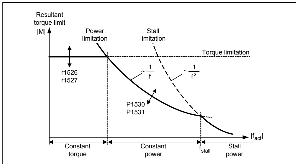
Fig. 3-109 Torque limits
