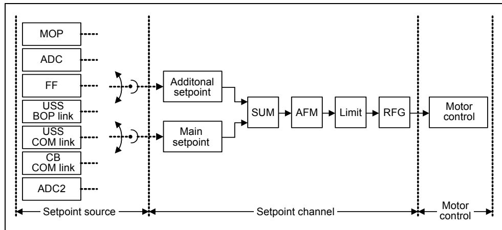
Fig. 3-59 Setpoint channel
