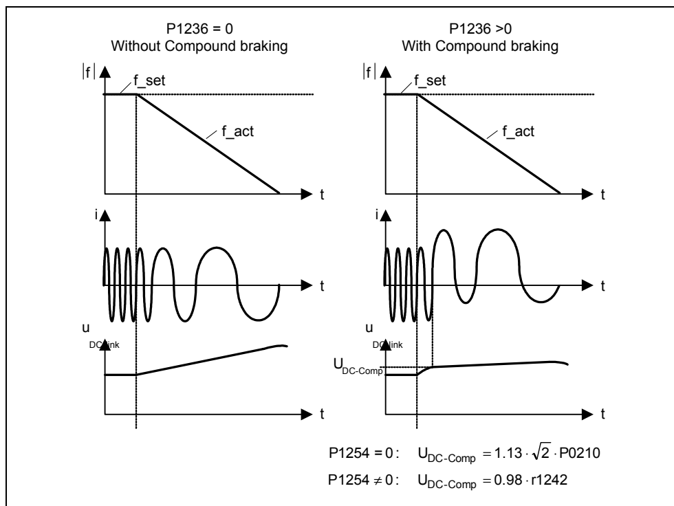
Fig. 3-75 Compound braking
