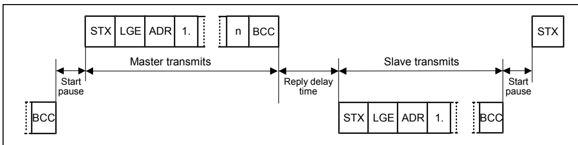
Fig. 3-43 Transmit sequence
