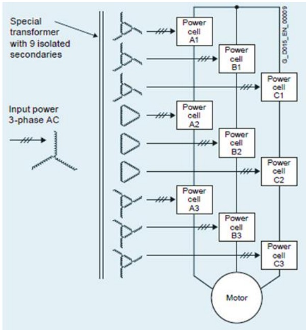
Figure 1: Topology of SINAMICS PERFECT HARMONY GH180 Drive (3 cells per phase)
