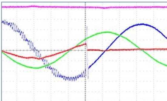
Figure 12: Optimized Synchronous Up Transfer
