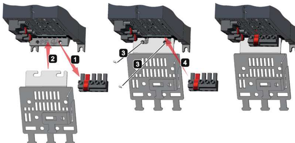
Figure 4-15 Mounting the shield connection plate on the PM240-2
