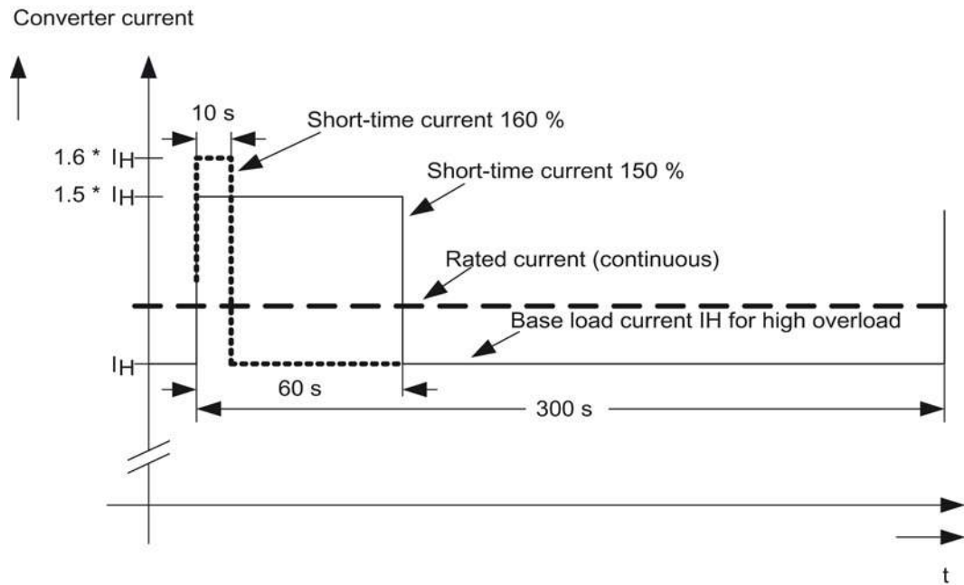
Figure 4-65 Characteristic: High overload
