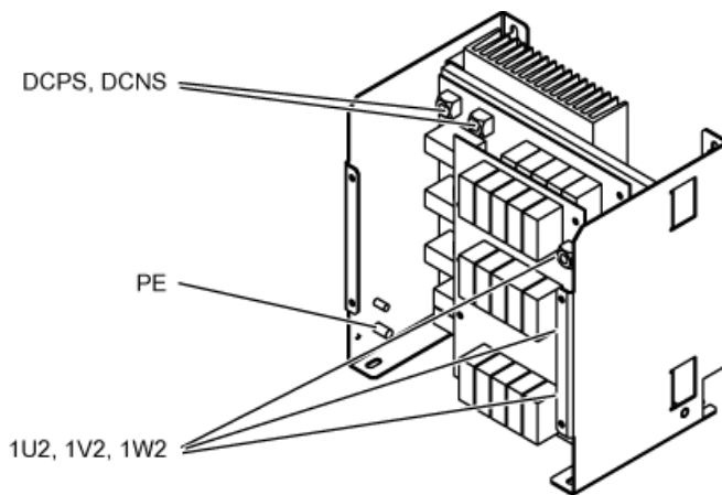
Figure 6-16 Interface overview, Voltage Peak Limiter, type 1
