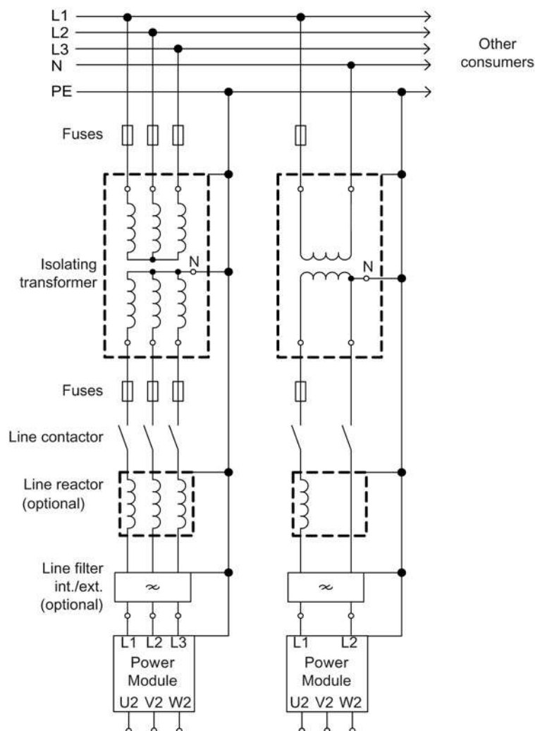
Figure 3-33 Isolating transformer
