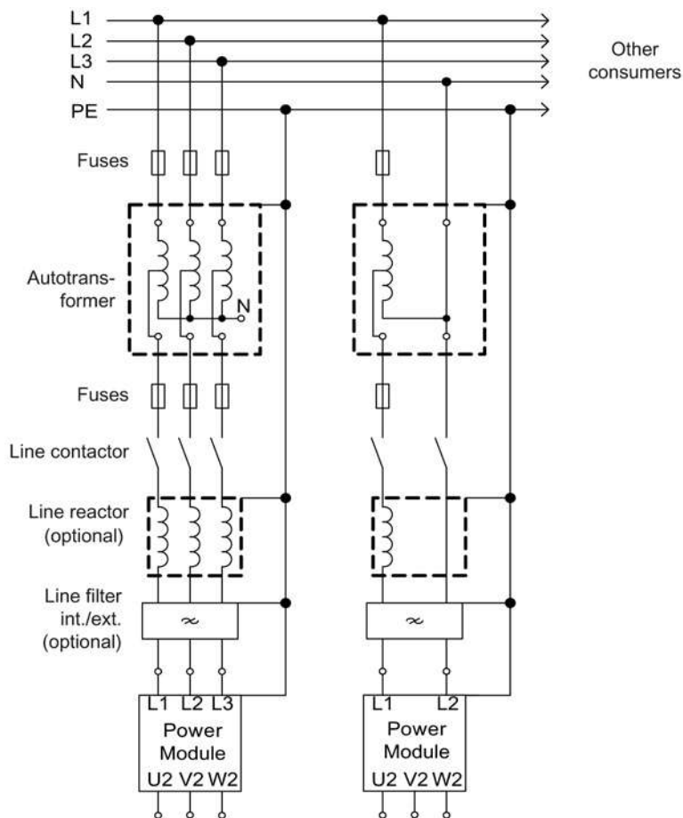
Figure 3-32 Auto-transformers
