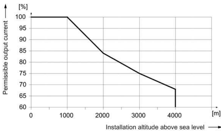
Figure 4-25 Output current as a function of the installation altitude
