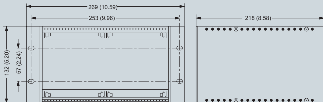
Transmitter back of panel, 42 TE
