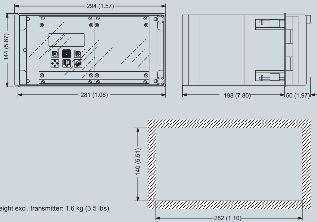
Transmitter, panel front IP65/NEMA 4, 42 TE
