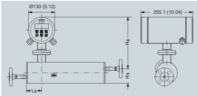
MASS 2100 and MASS 6000 Ex d compact version
