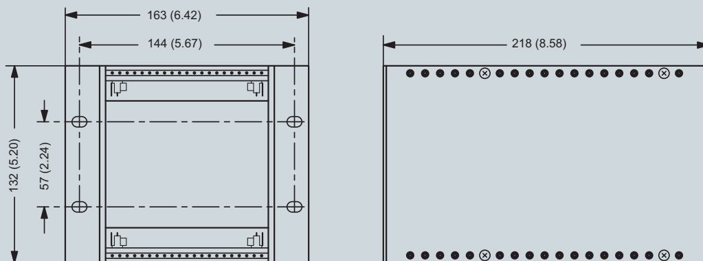
Transmitter back of panel
