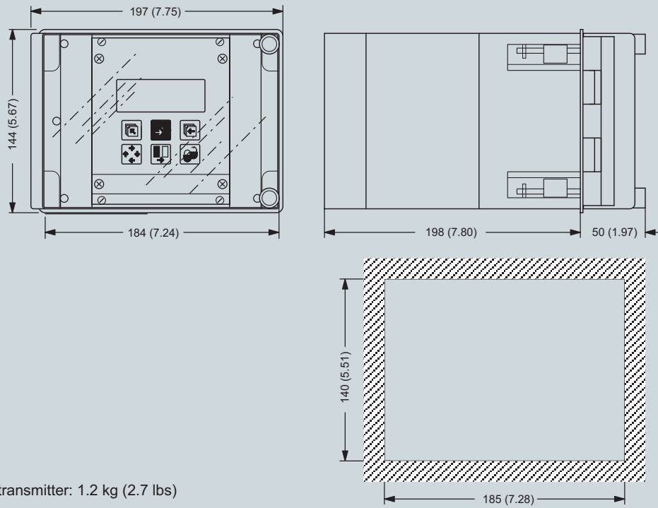
Transmitter, panel front IP65/NEMA 4, 21 TE
