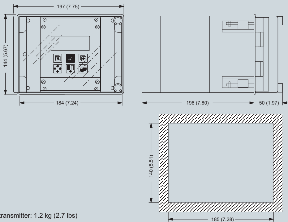
Transmitter 19" front of panel
