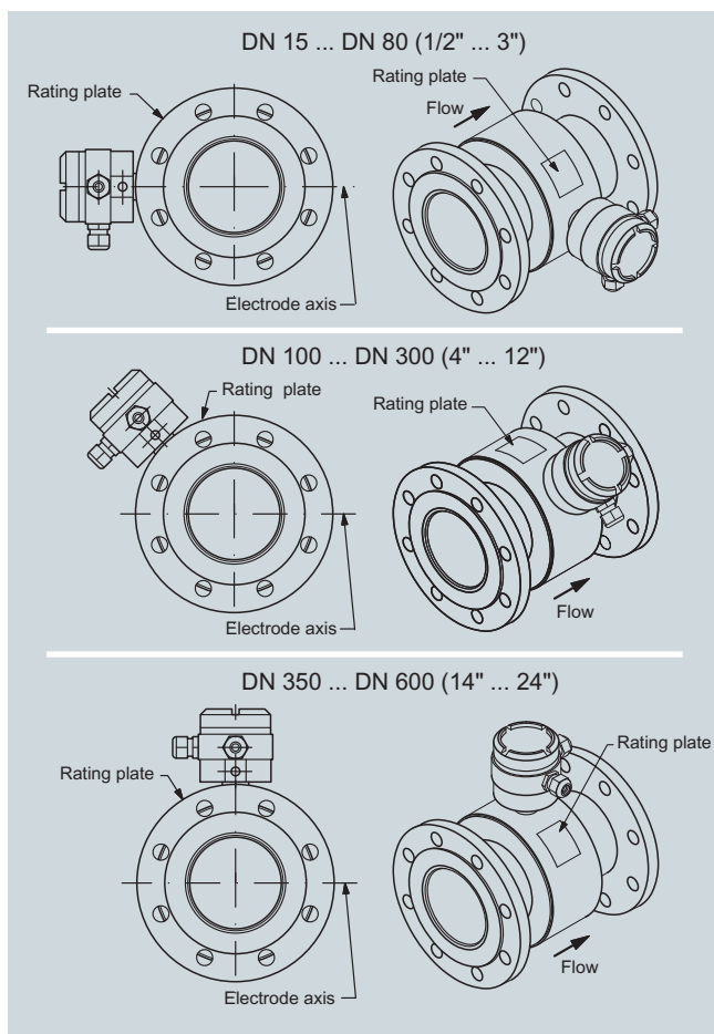
Electrode placement
