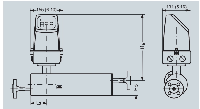
MASS 2100 and MASS 6000 IP67 compact version
